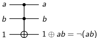
Figure 10: NAND gate.
