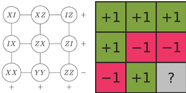
Figure 4: Mermin-Peres square.
